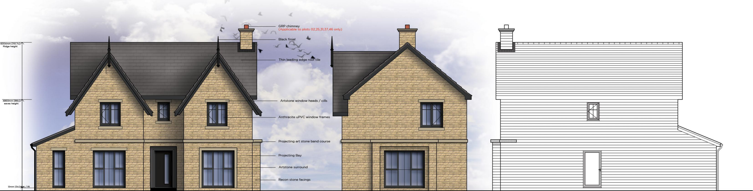
Front Elevation
